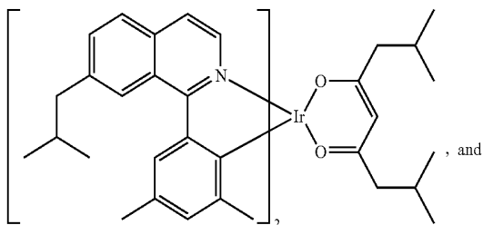
Compound 6
