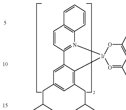
Compound 5
