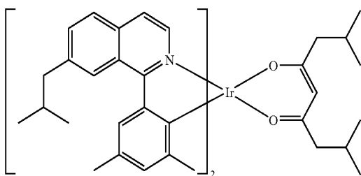
Compound 7
