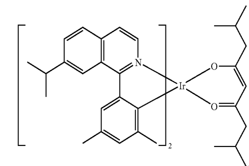
Compound 7
