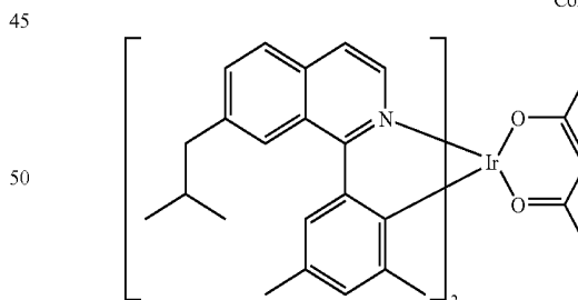
Compound 10
